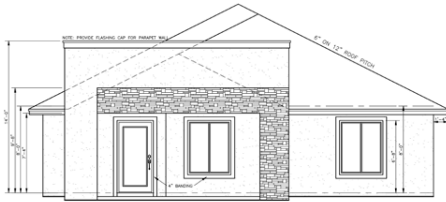
Front Elevation
