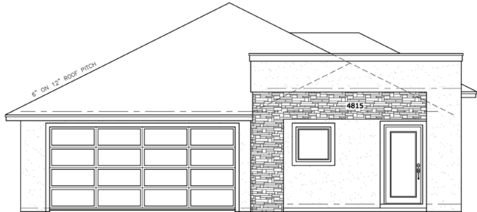
Front Elevation
