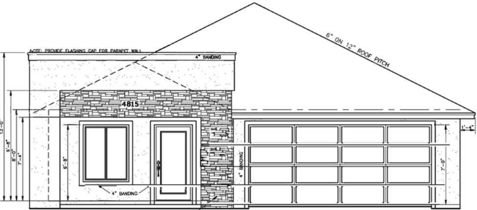
Front Elevation
