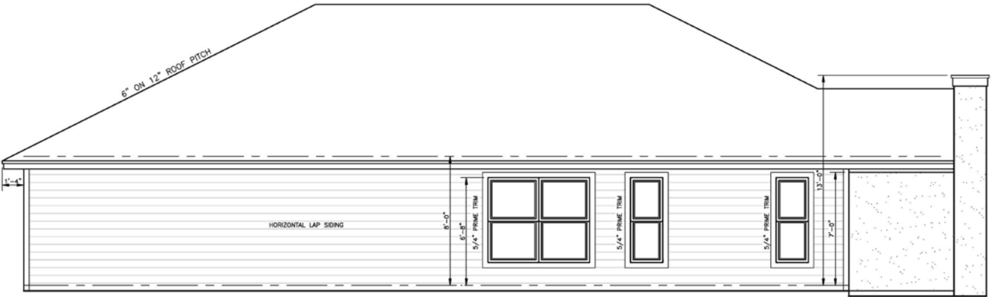
Left Elevation
